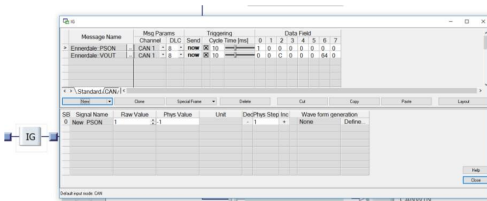
Figure 15 CANalyzer window
